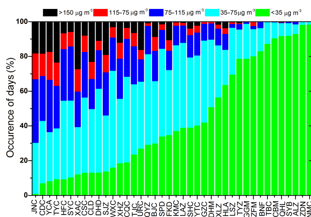
Figure 6. Days separated by the threshold values of the Ambient Air Quality Standard (AAQS) (GB3095-2012) of the Chinese guidelines. The threshold values of 35, 75, 115 and 150 µg m -3 used for the daily concentration ranges are represented as clean (< 35 µg m -3 ), slightly polluted (35–75 µg m -3 ), moderately polluted (75–115 µg m -3 ), polluted (115–150 µg m -3 ) and heavily polluted (> 150 µg m -3 ), which was suggested by the AAQS guidelines. The site codes related to the observation stations can be found in Table 1.
