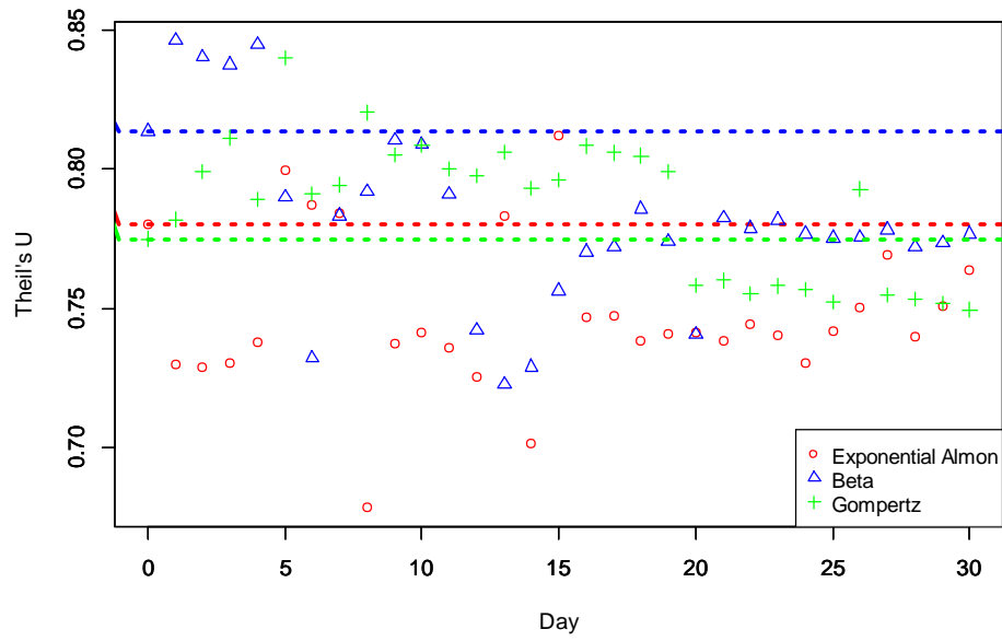
Fig. 8. Theil's U of nowcasting for the MIDAS-SARIMA models with different weighting schemes.
