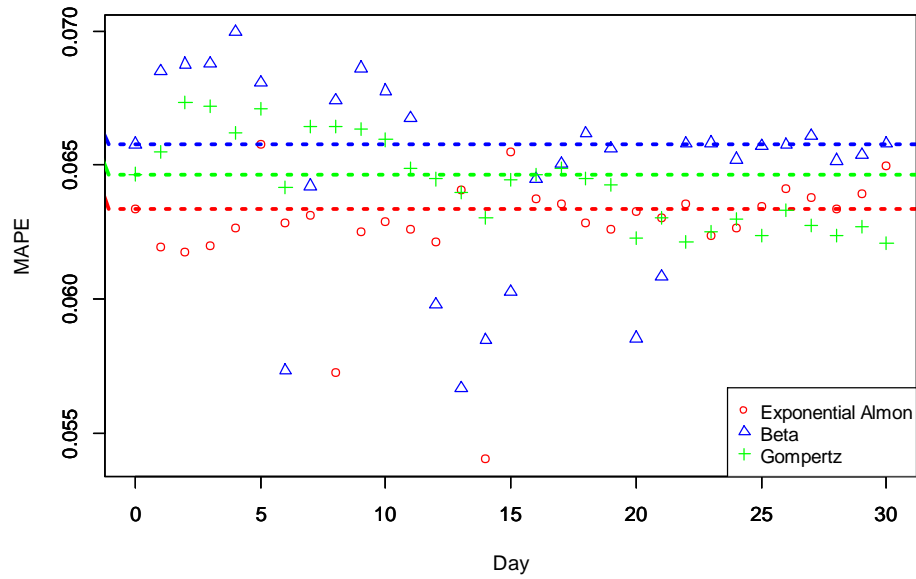
Fig. 6. MAPE of nowcasting for the MIDAS-SARIMA models with different weighting schemes.
