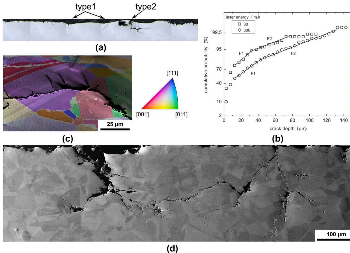
Fig. 23. Stress corrosion cracking (SCC) in laser-processed stainless steels. (a) Type 1 (from surface) and type 2 (from corrosion pits) SCC in 305 stainless steel (synthetic seawater, 1500 h). (b) Crack depth is limited by the extent of tensile residual stress, influenced by laser energy. (c) EBSD map showing transgranular SCC in 316L stainless steel (MgCl 2 3950 \mu\text{g}/\text{cm}^2 , 402 days). (d) local corrosion and SCC networks in 316L stainless steel. (a)–(b) taken from Eto et al. [149], (c)–(d) taken from Krawczyk et al. [151].
