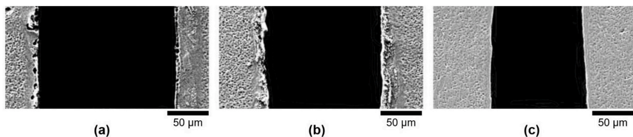
Fig. 22. Acid-etched (HF/HNO 3 ) laser cut TC1 sheet with different assist gases: (a) air, (b) N 2 , and (c) Ar. Corrosion of recast layer is reduced on Ar flushing. Taken from Shanjin and Yang [140].
